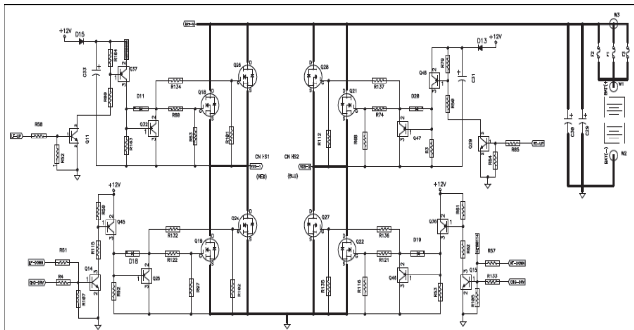
Figure S-5 Inverter circuit
