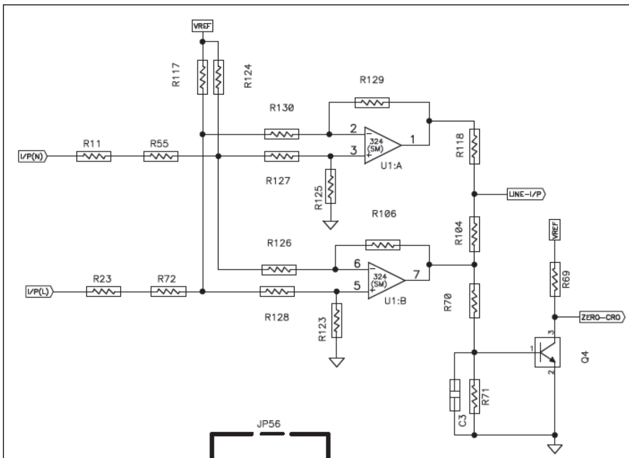
Figure S-4 Line and Zero Crossing Detecting Circuit
