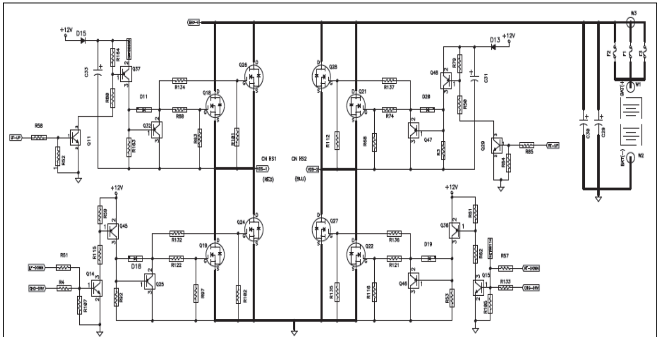
Figure S-3-B Charger Control Circuit
