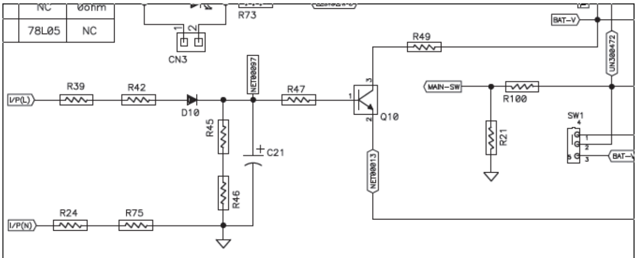
Figure S-2-3 AC start Circuit
