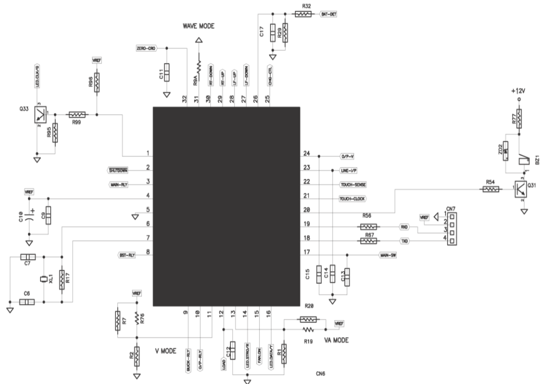
Figure S-6 CPU Control Circuit
