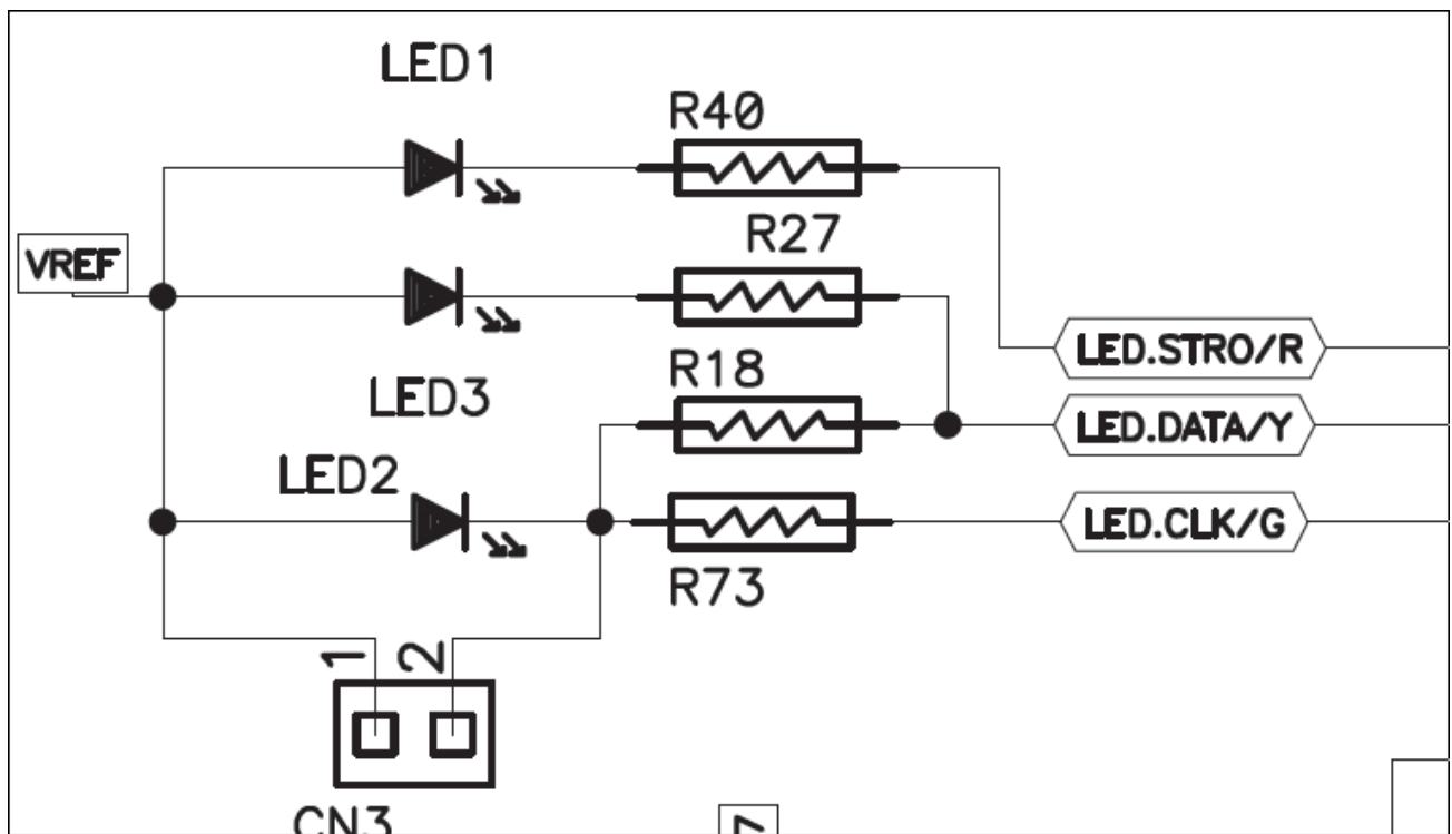
Figure S-8 Display Circuit
