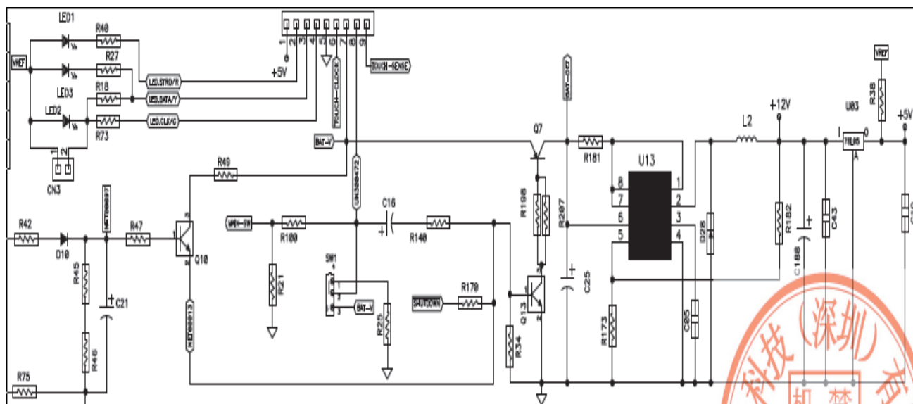
Figure S-2-1 Control Power Circuit (+12Vdc)
