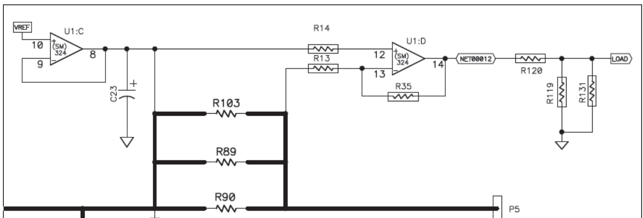
Figure S-9 Load Detection Circuit
