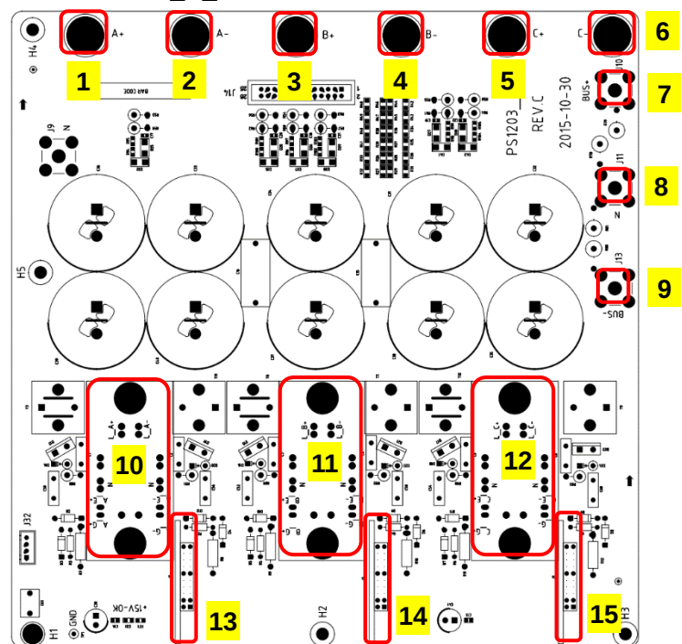
Fig. 3-9 PFC board assembly diagram
