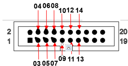
Sampling resistance detection Tab.3-6-5
