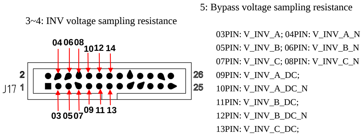
Fig.3-17 Detect area (J17 port PIN)
