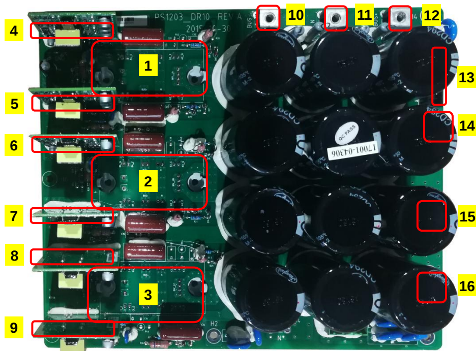
Fig.3-12 Inverter board introduction
