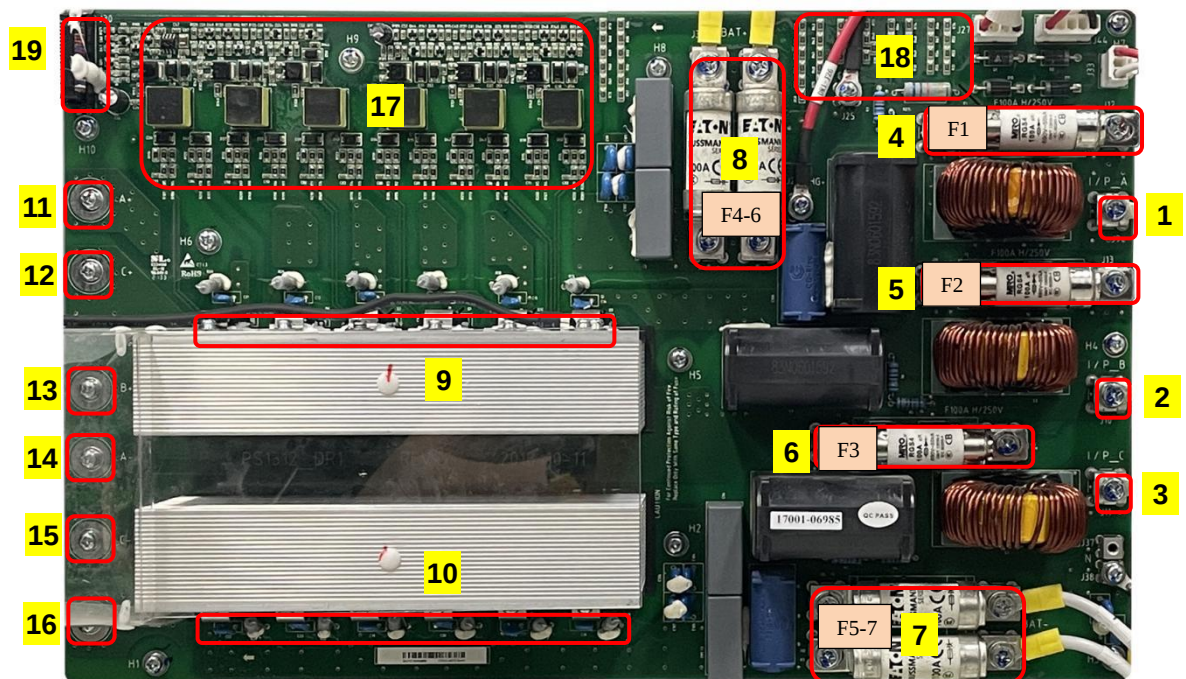
Fig.3-3 Input SCR board introduction
