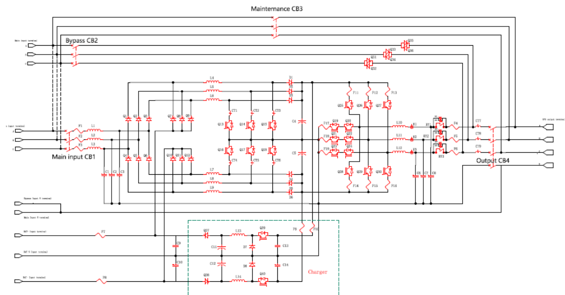
Fig.2-2 NOVA 30 topology
