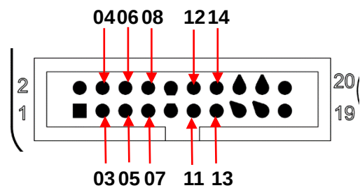
Fig.3-6 Detect area (J30 port PIN)
