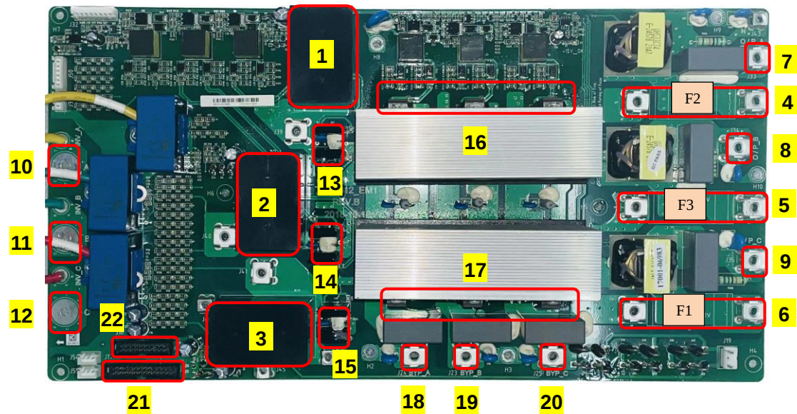
Fig.3-14 Output board introduction
