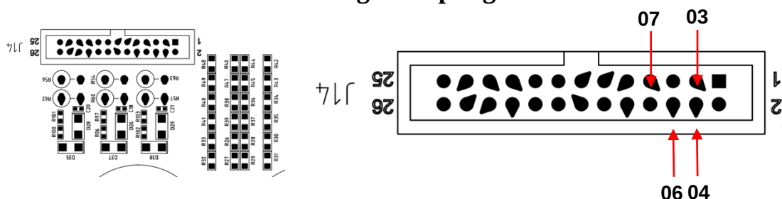
Fig.3-10 Detect area (J14 port PIN)
