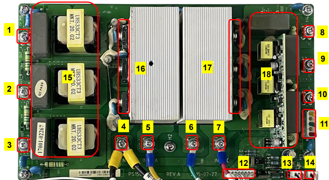
Fig.3-22 Bypass SCR board introduction
