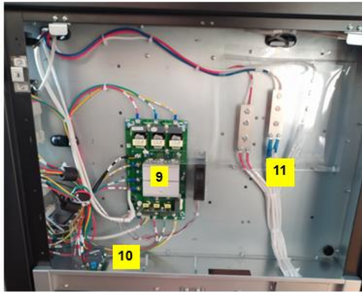
Fig.1-3 Left side structure
