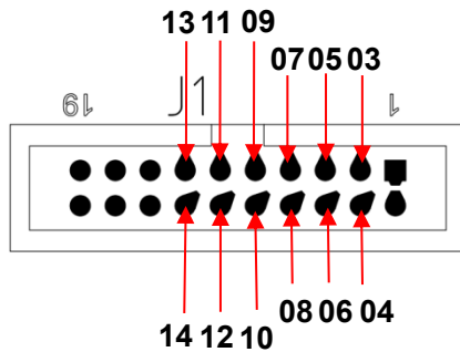
Fig.3-17 Detect area (J1 port PIN)
