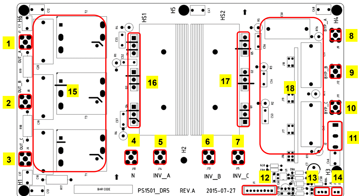
Fig.3-23 Bypass SCR board assembly diagram
