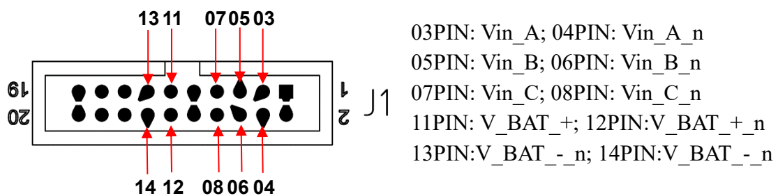
Fig.3-6 Detect area (J1 port PIN)
