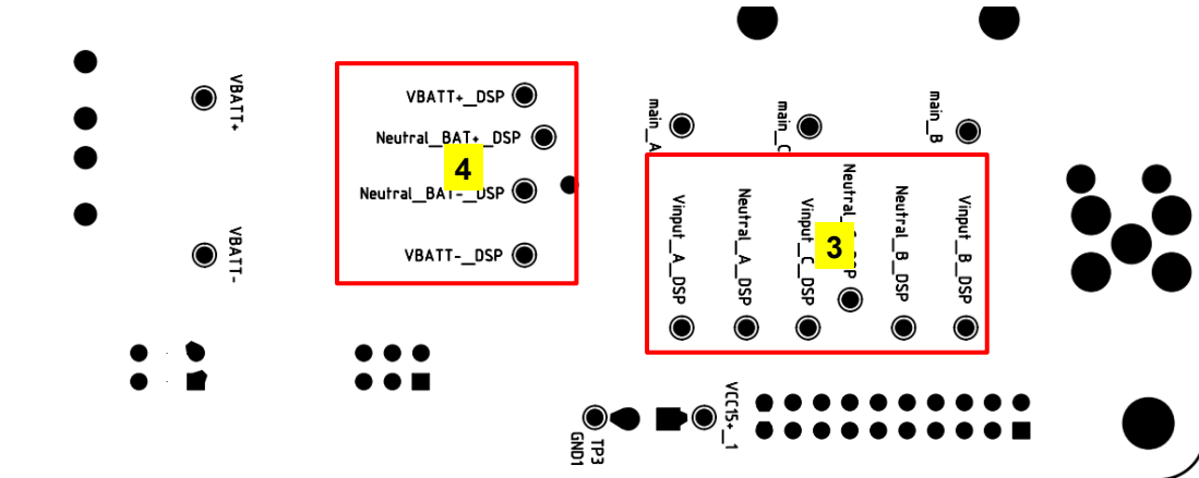
Fig.3-7 Detect area (back of the input board)
