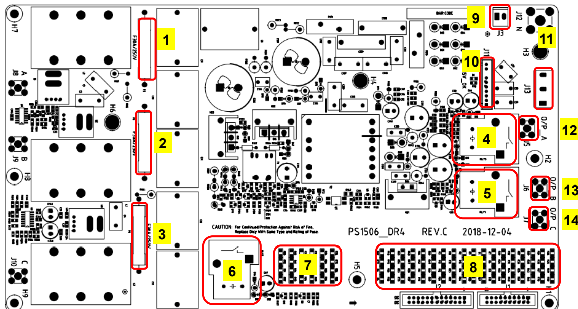
Fig.3-15 Output board assembly diagram
