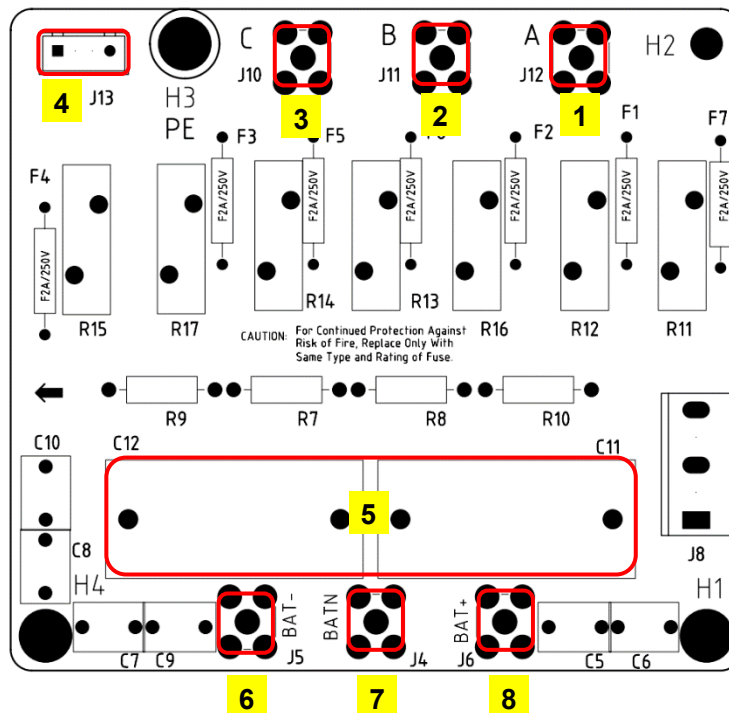
Fig.3-27 Battery EMI and lighting protection board assembly diagram
