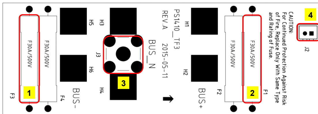
Fig.3-21 Inverter bus board assembly diagram
