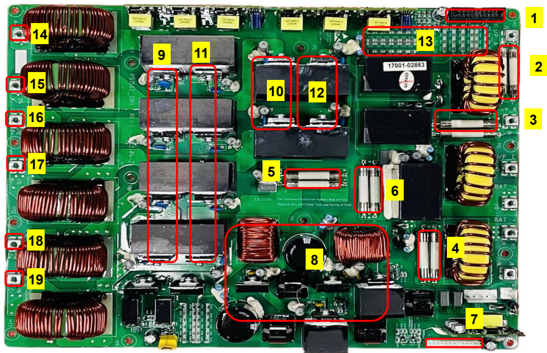
Fig.3-3 Input SCR board introduction
