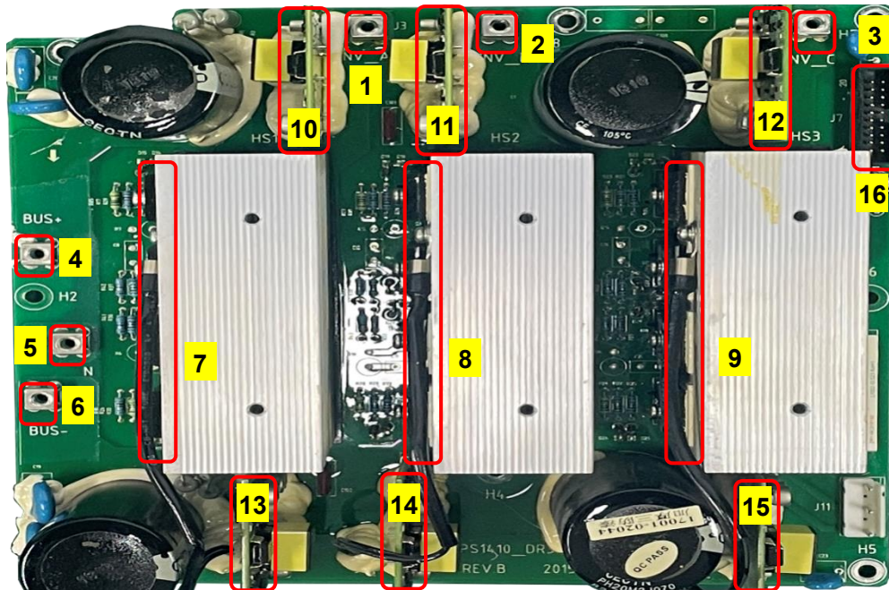
Fig.3-12 Inverter board introduction
