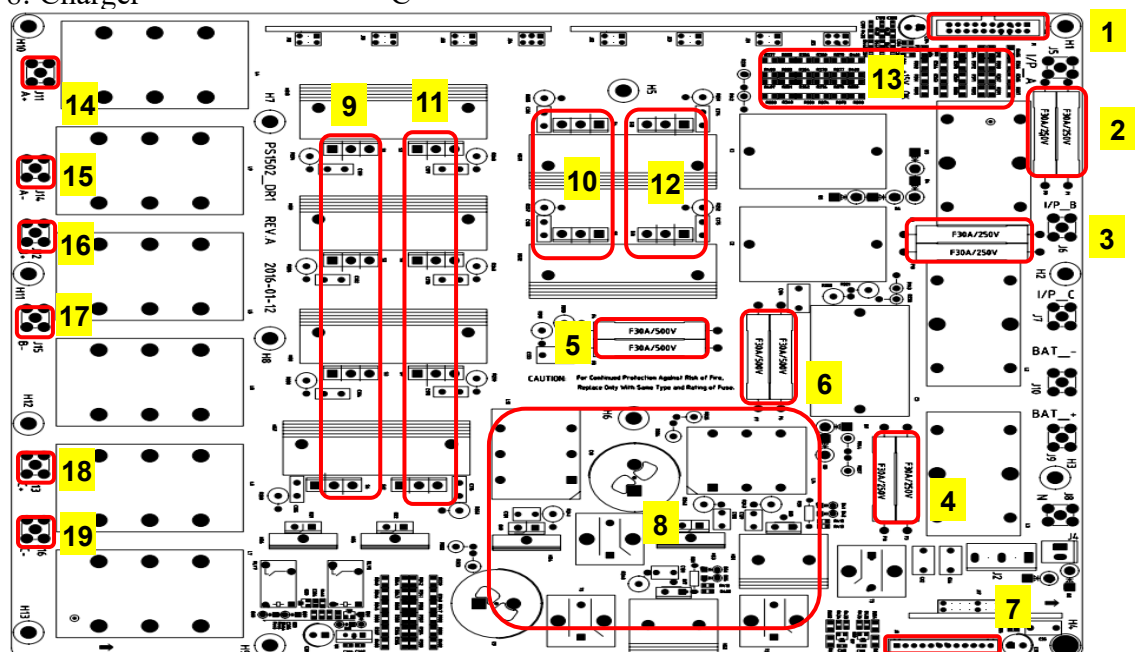
Fig.3-4 Input SCR board assembly diagram
