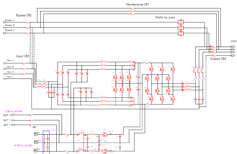
Fig.2-2 NOVA 15K topology
