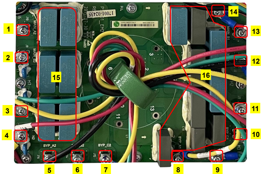
Fig.3-24 Input EMI board introduction
