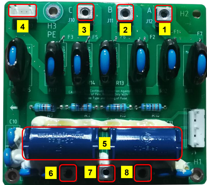
Fig.3-26 Battery EMI and lighting protection board introduction
