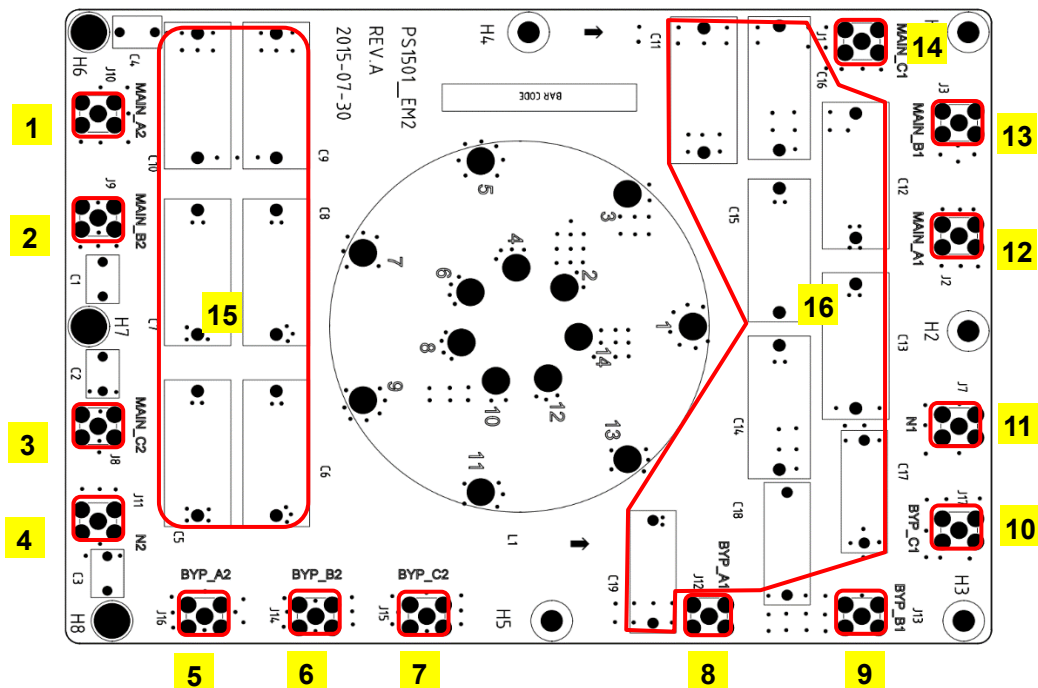
Fig.3-25 Input EMI board assembly diagram
