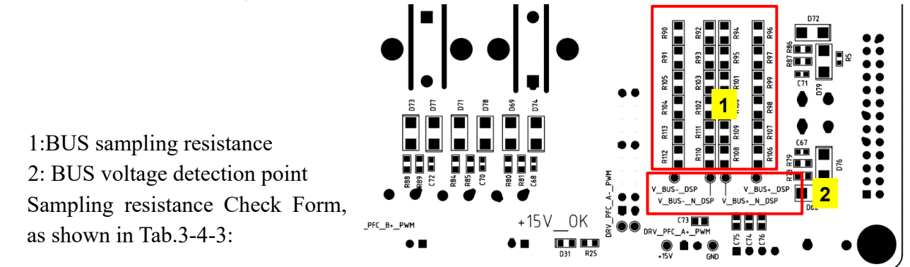
Fig.3-11 Detect area (back of the PFC board)
