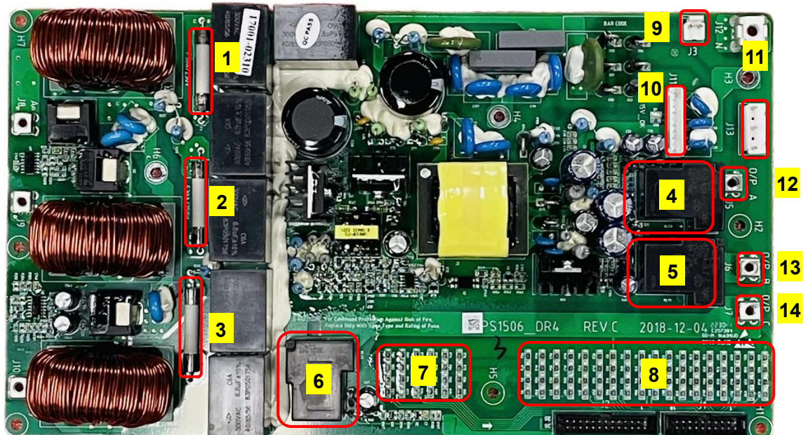
Fig.3-14 Output board introduction
