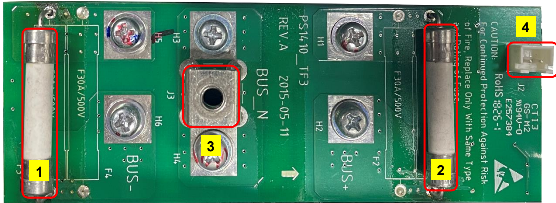
Fig.3-20 Inverter bus board introduction
