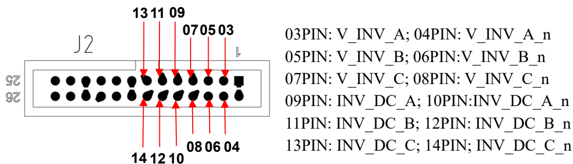
Fig.3-18 Detect area (J2 port PIN)
