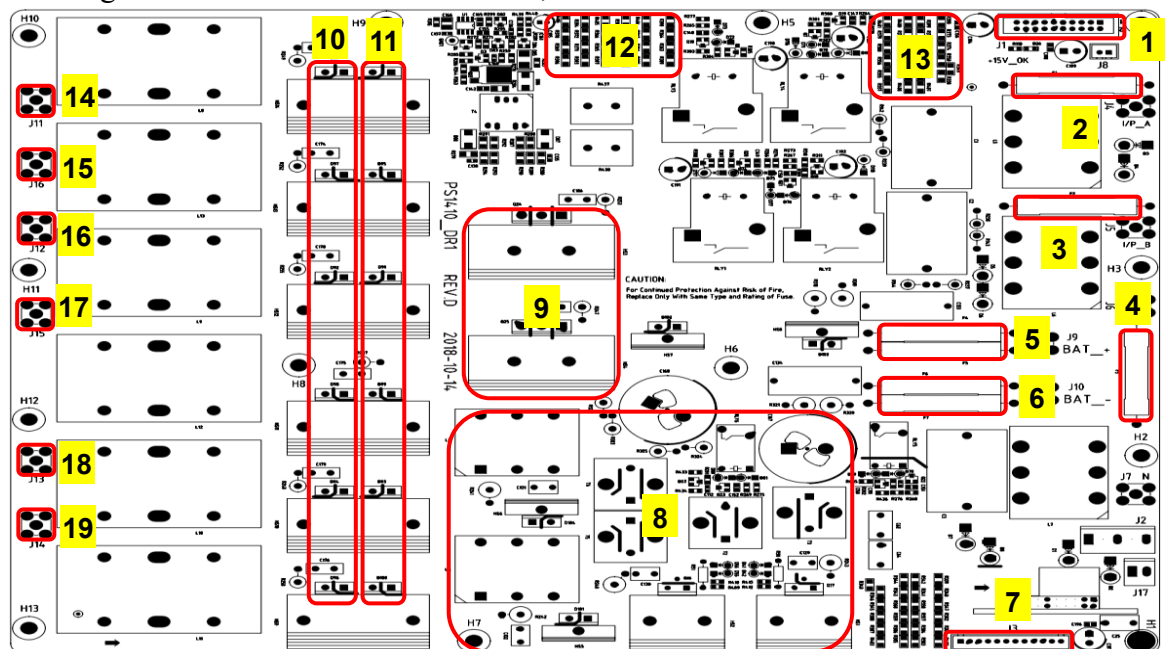
Fig.3-4 Input SCR board assembly diagram
