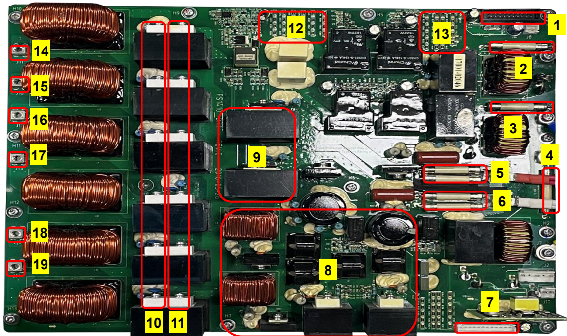
Fig.3-3 Input SCR board introduction
