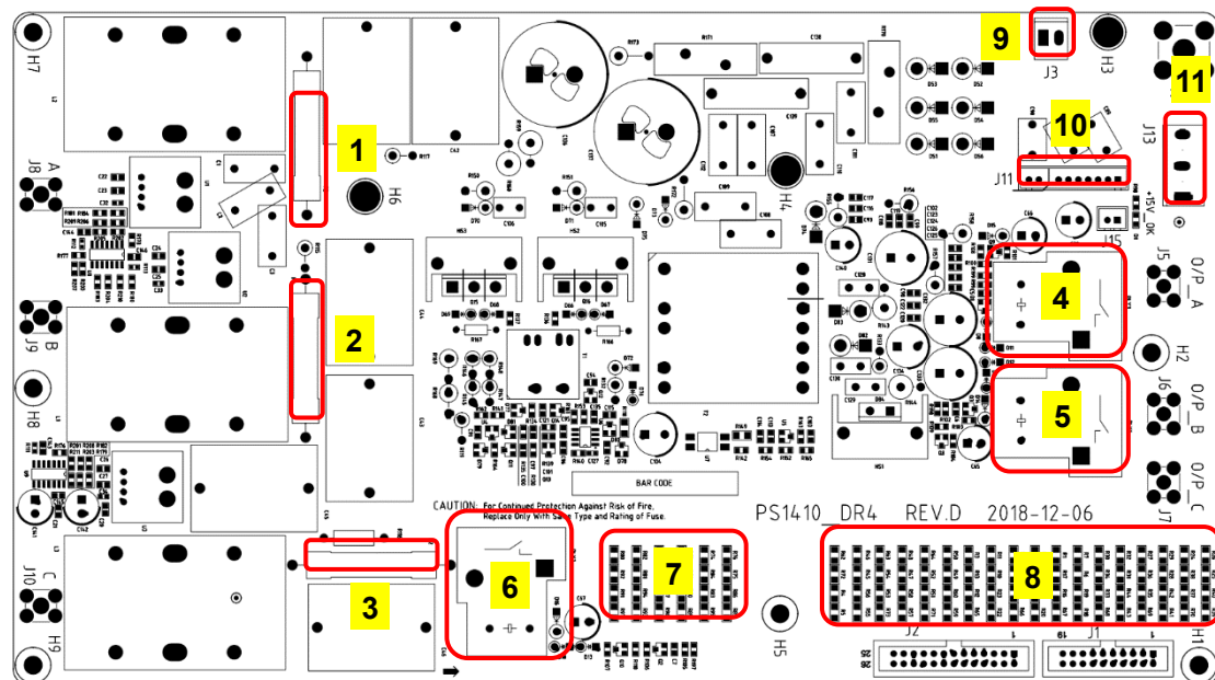
Fig.3-15 Output board assembly diagram
