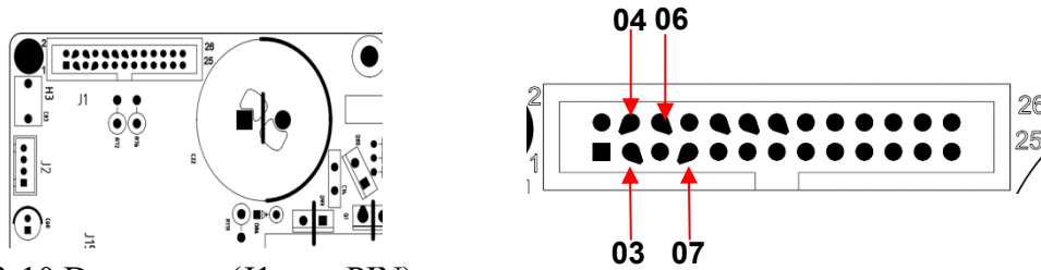
Fig.3-10 Detect area (J1 port PIN)
