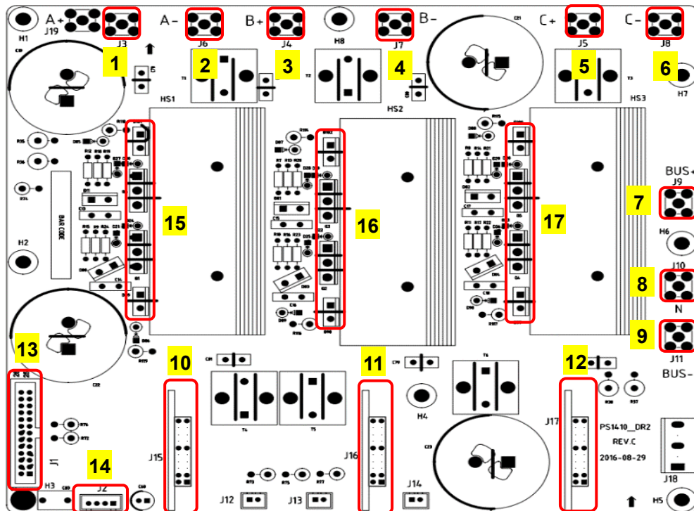
Fig. 3-9 PFC board assembly diagram
