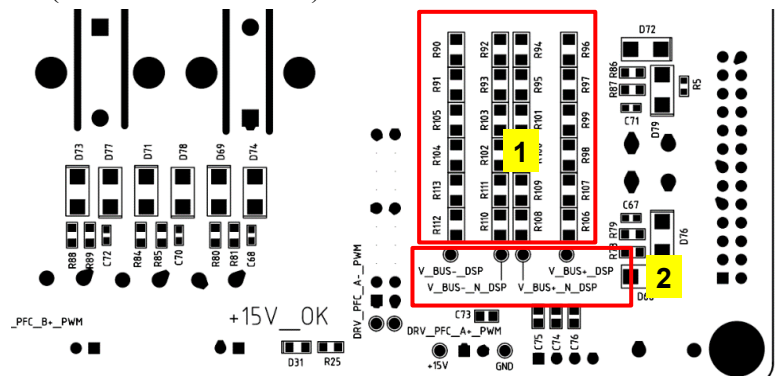
Fig.3-11 Detect area (back of the PFC board)
