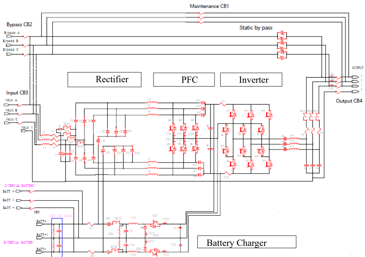
Fig.2-1 Uninterruptible Power Supply schematic diagram
