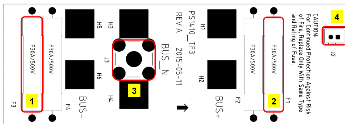
Fig.3-21 Inverter bus board assembly diagram
