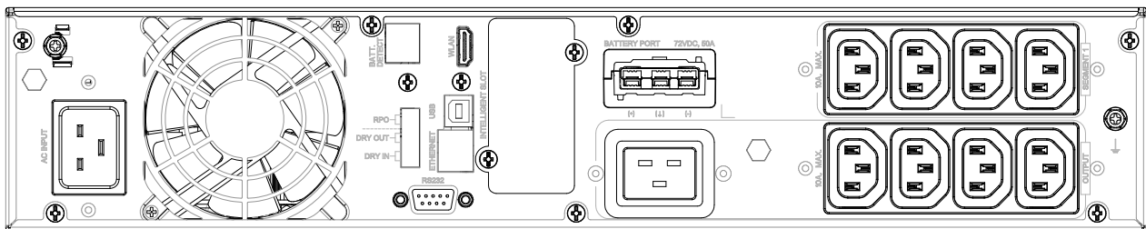
3K REAR PANEL
