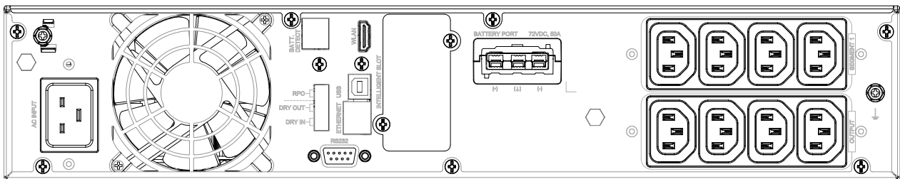
2K REAR PANEL
