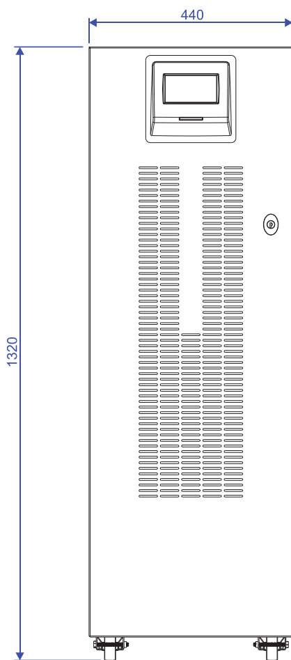
FRONT VIEW
