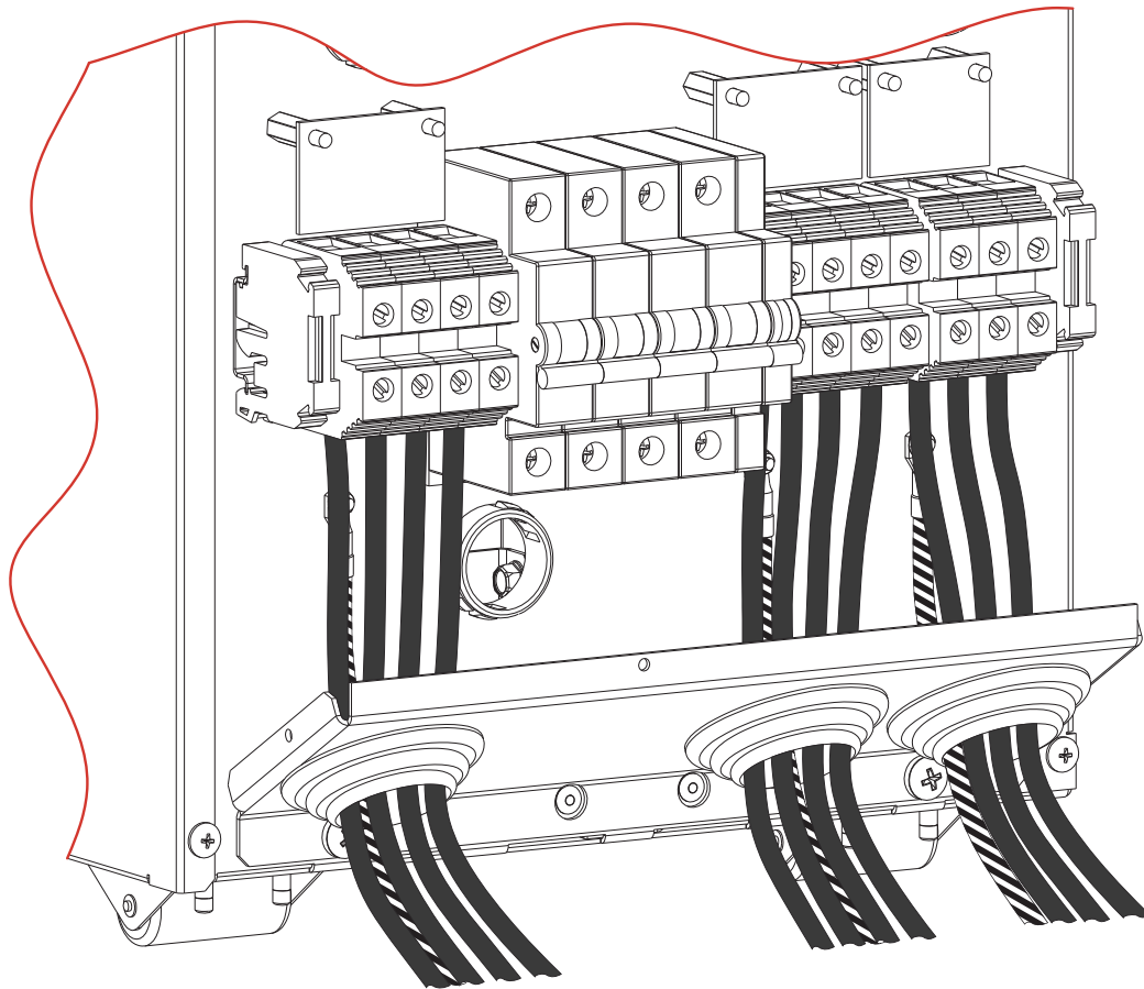
CABLE POSITION DETAIL
