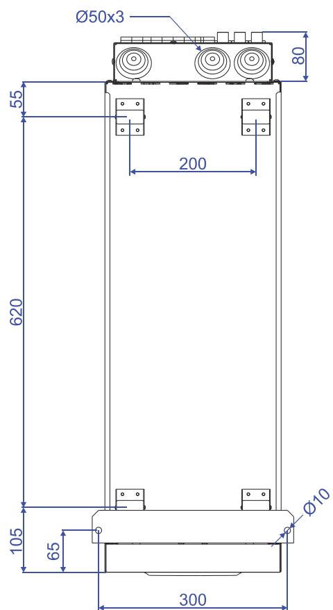
BOTTOM VIEW
