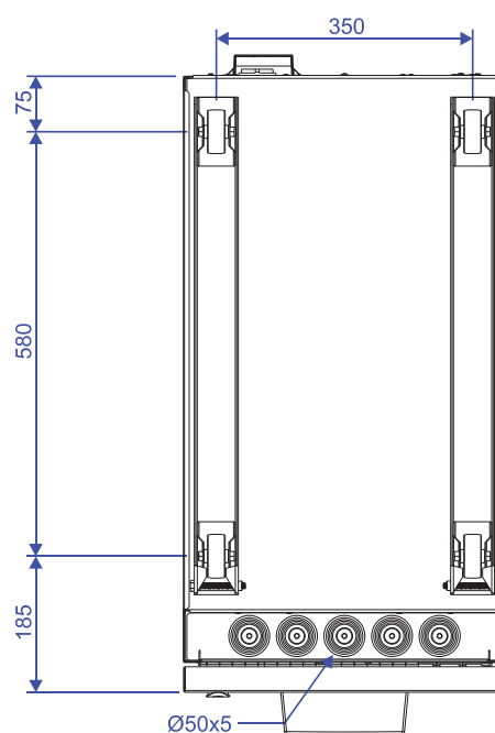
BOTTOM VIEW
