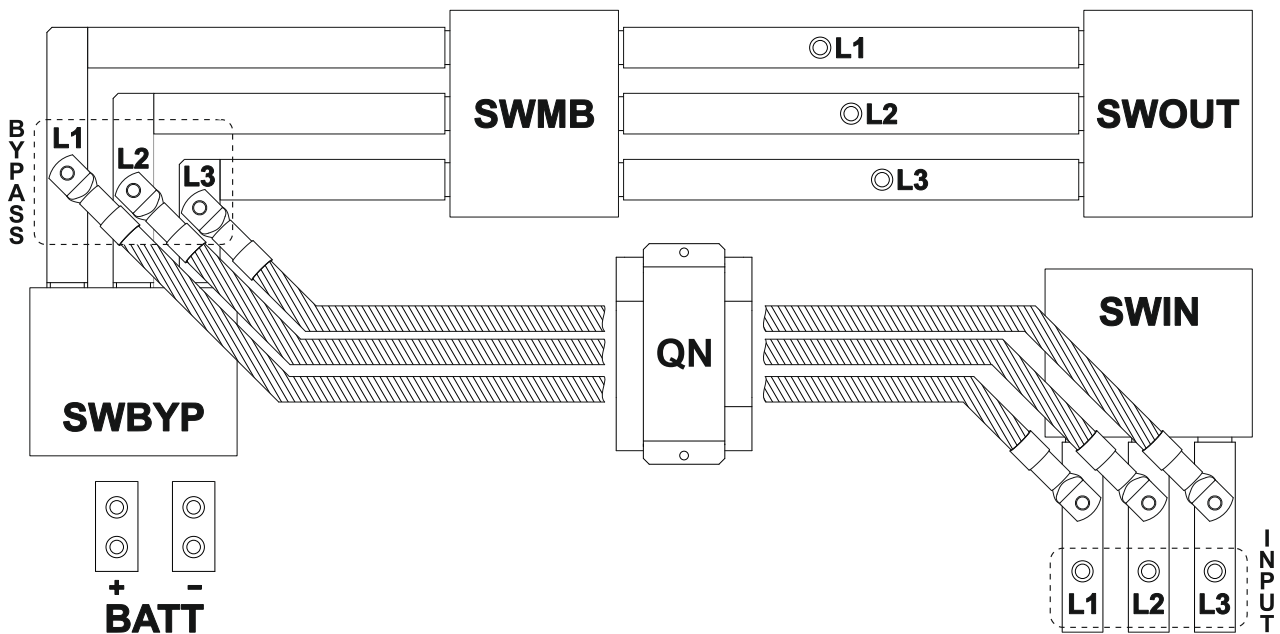
125KVA - BYPASS CONNECTED TO INPUT LINE
