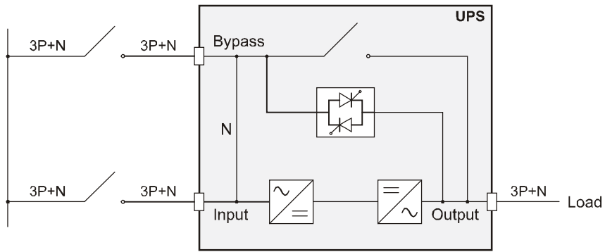
UPS without neutral connectivity variation and with separate bypass input
