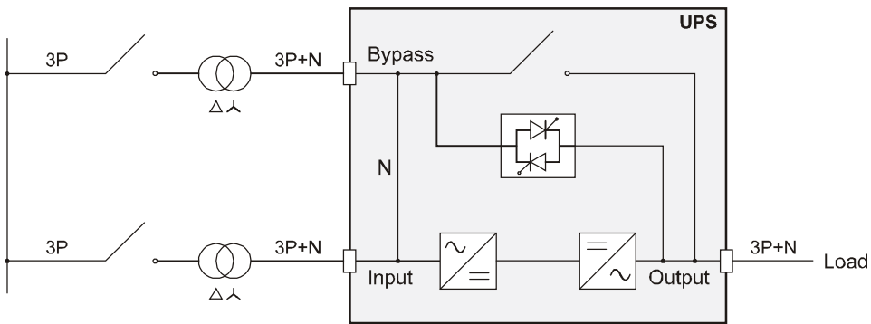
UPS with galvanic input insulation and with separate bypass input
