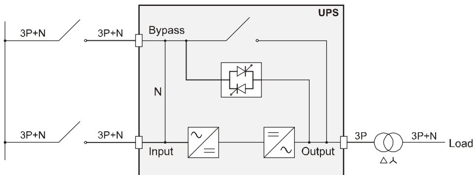
UPS with galvanic output insulation and with separate bypass input
