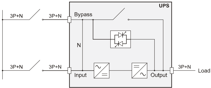
UPS without neutral connectivity variation and with separate bypass input
