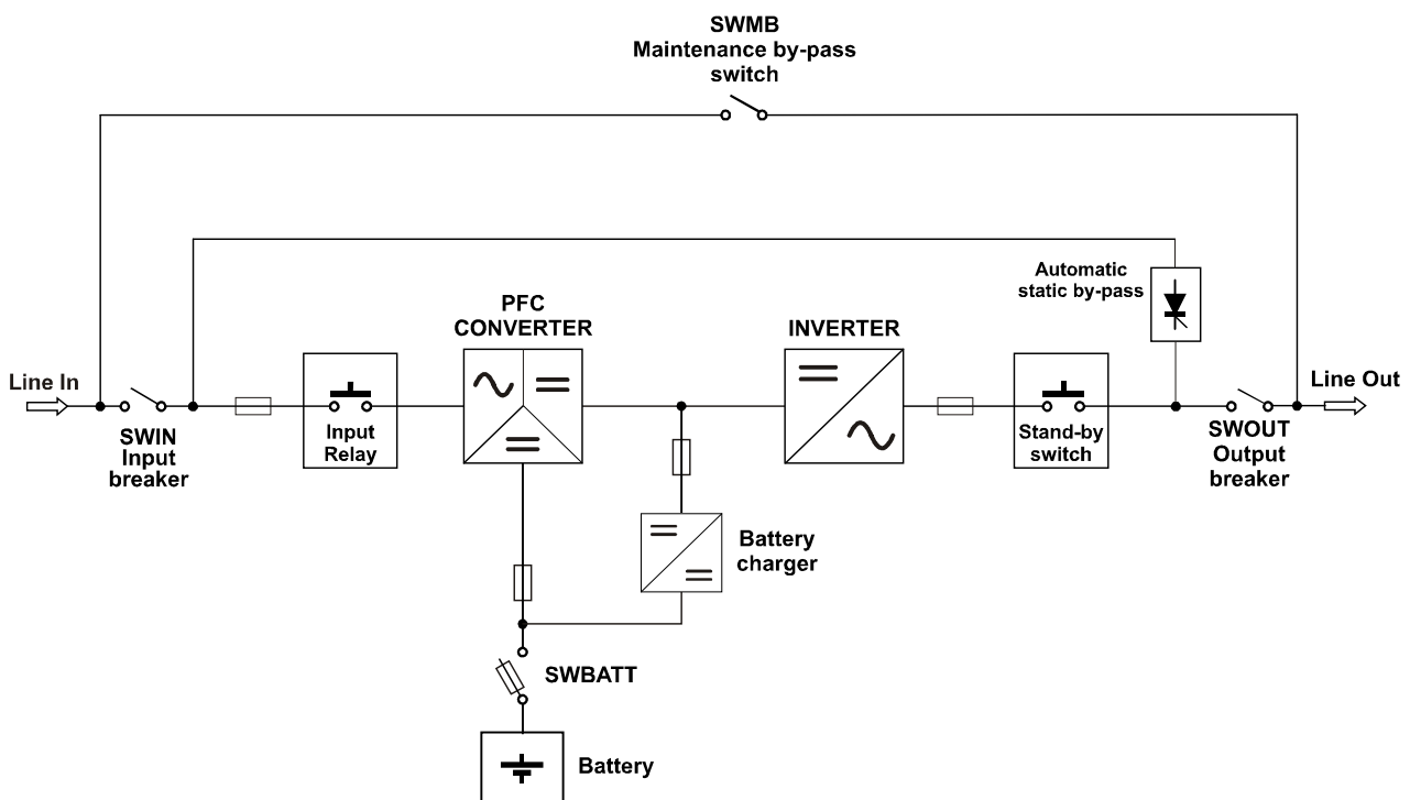
Block diagram of the UPS
