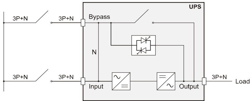
UPS without any variation in neutral condition and with separate bypass iut
