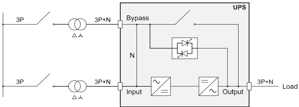
UPS with galvanic isolation and with separate bypass iut
