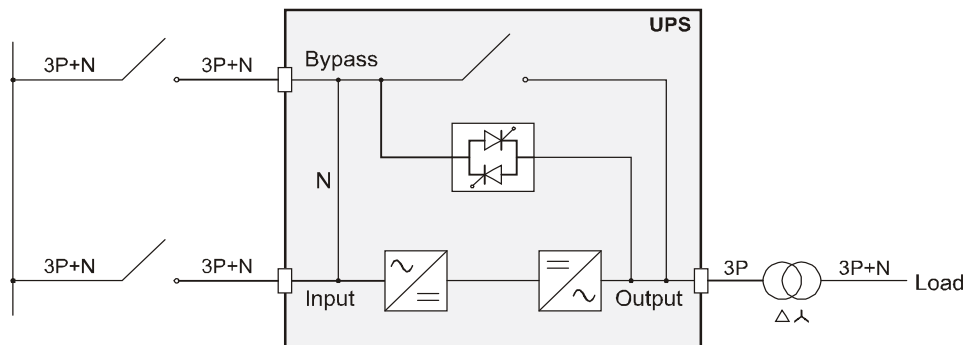
UPS with galvanic isolation at output and separate bypass iut
