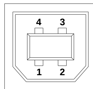
USB CONNECTOR
